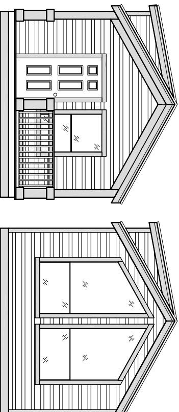
Optional Side Elevations
